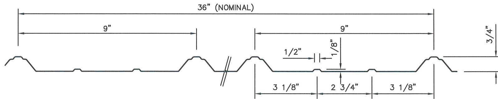
PANEL PROFILE
